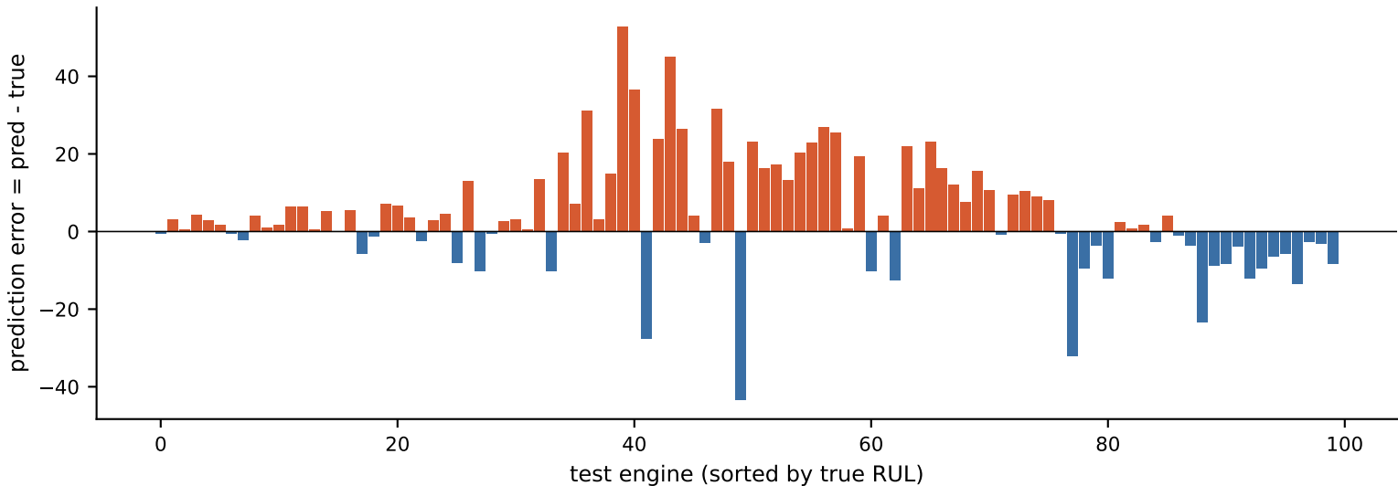
Per-engine LSTM prediction error on FD001 (red = late prediction, blue = early)
