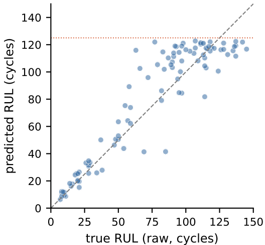
FD001 (RMSE=15.27)
