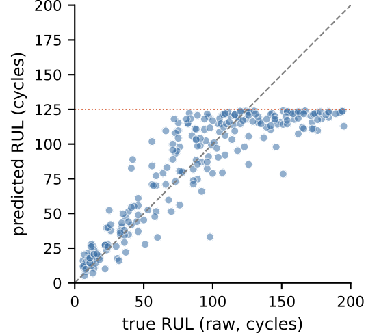
FD004 (RMSE=15.50)
