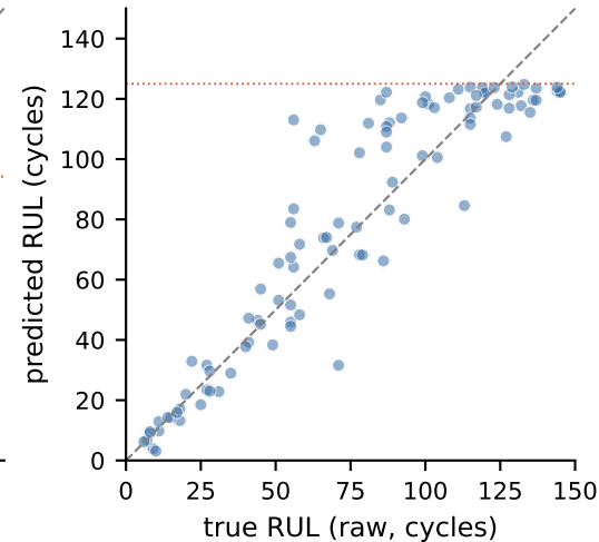
FD003 (RMSE=14.97)
