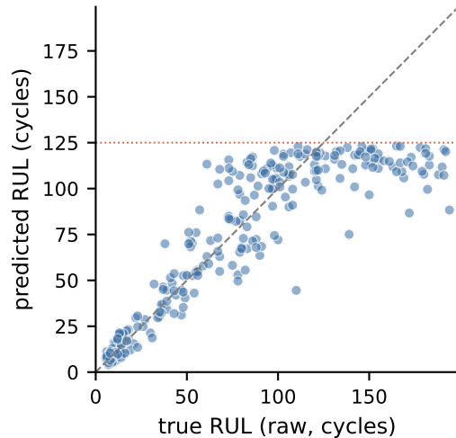
FD002 (RMSE=14.74)
