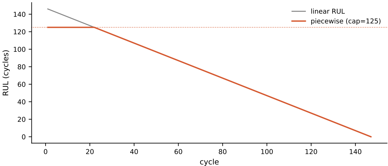
Linear vs piecewise-linear RUL target (FD001 engine 24)
