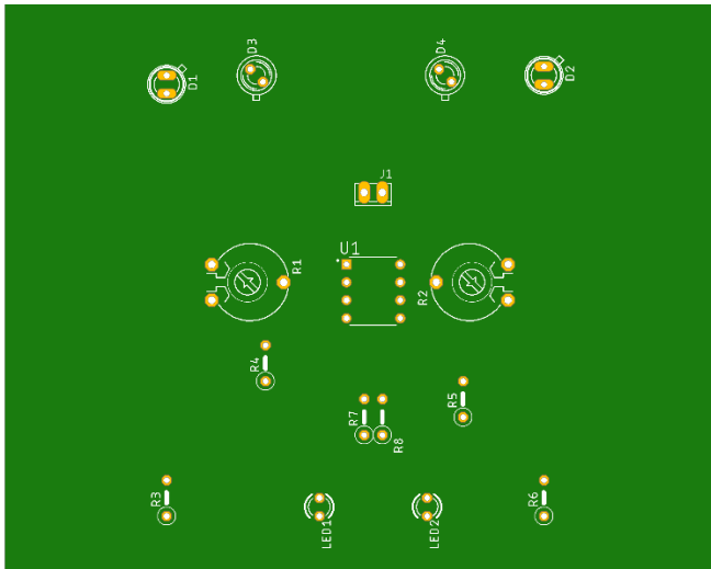
IR Circuit Manufacturing Top Side
