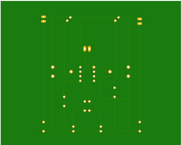
IR Circuit Manufacturing Bottom Side
