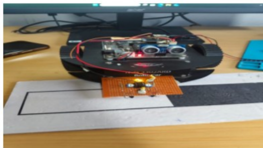
Fig. 5.11 Setup for testing of Receiver circuit when both IR pair on black surface
