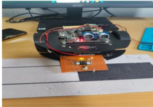
Fig. 5.10 Setup for testing of Receiver circuit when One IR pair on black and other on white surface
