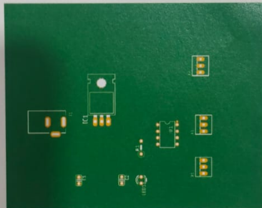
Transmitter Circuit Manufacturing Top Side
