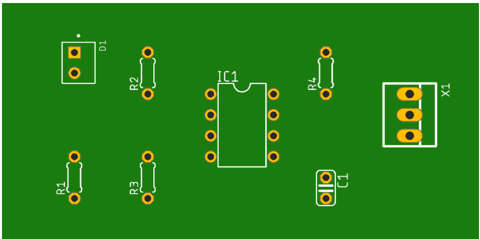
Receiver Circuit Manufacturing Top Side
