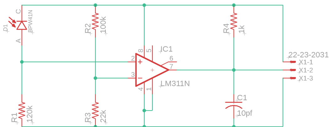
Receiver Circuit Layout
