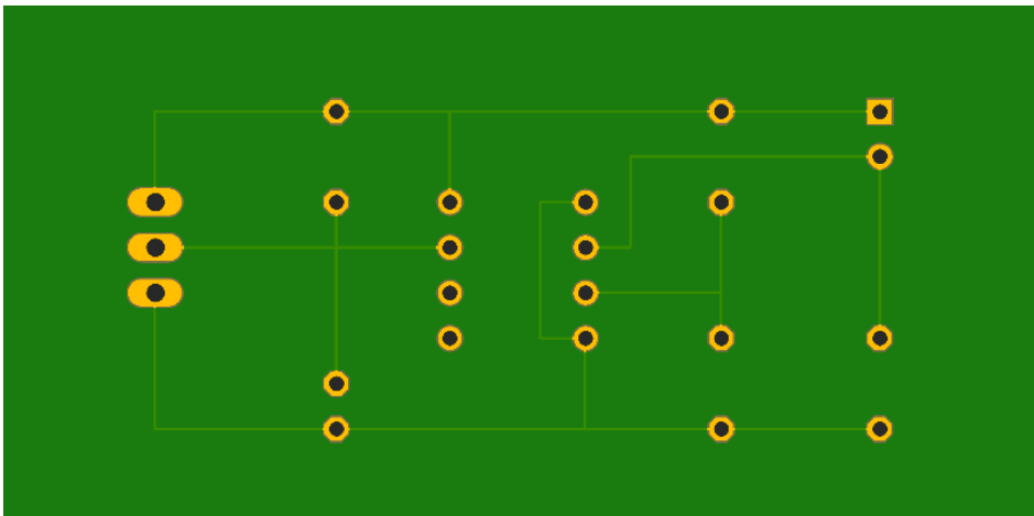
Receiver Circuit Manufacturing Bottom Side
