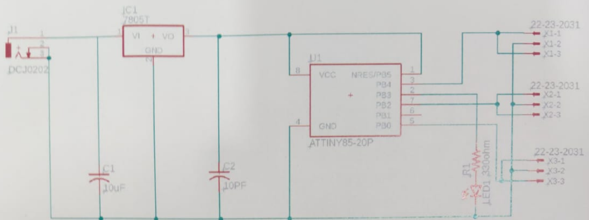
Transmitter Circuit Layout
