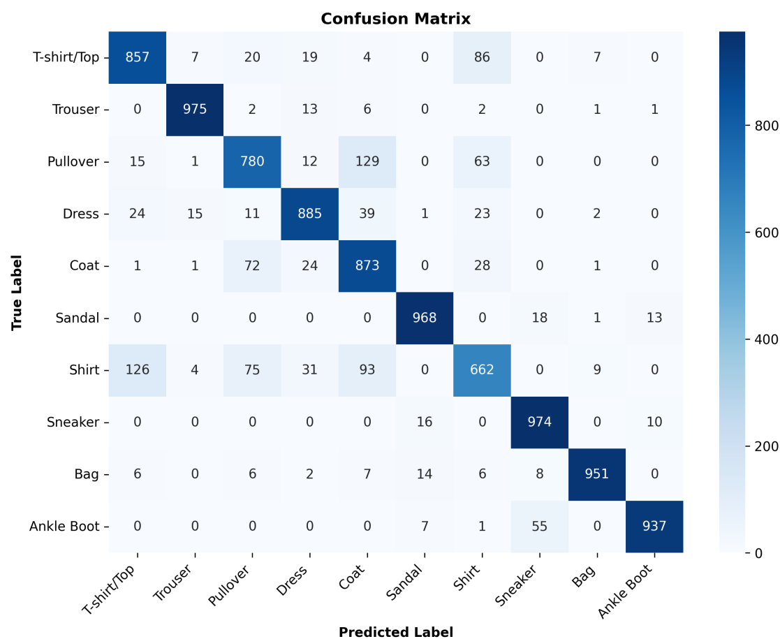
Figure 5: Confusion Matrix
