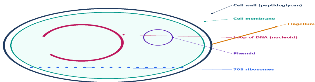
Typical prokaryotic cell (not to scale)
