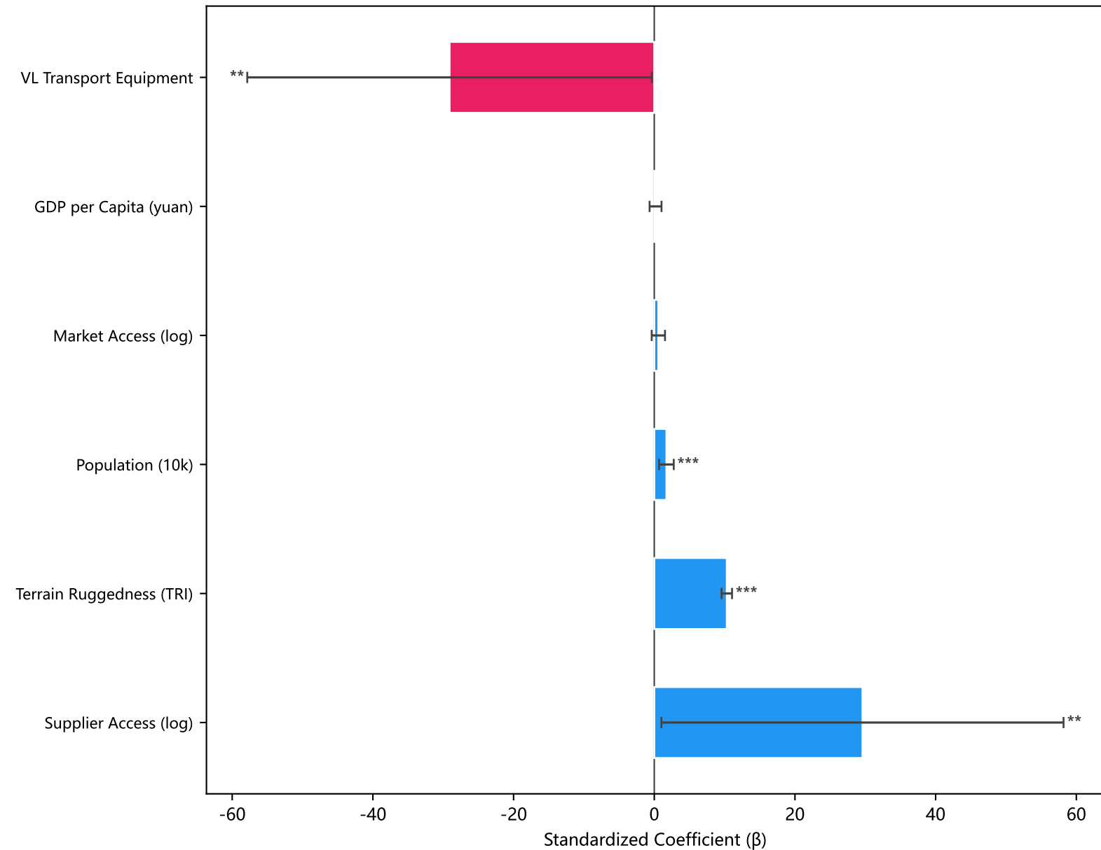
B. OLS Coefficient Estimates (2023 Cross-Section)
