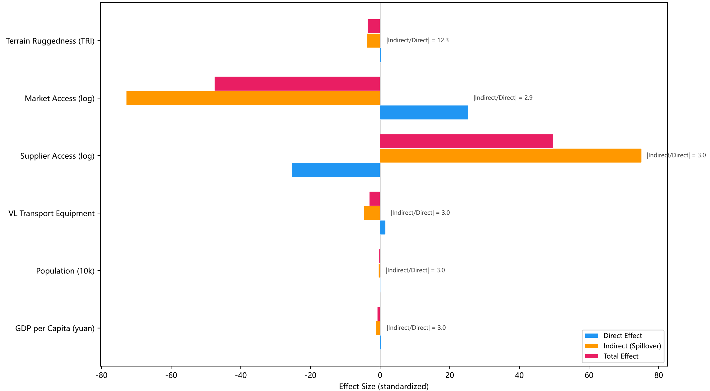
Spatial Durbin Model: Direct, Indirect & Total Effects (2023)
