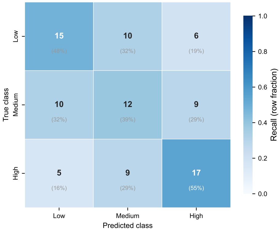
Confusion Matrix — GCN (OD) (N = 93, 3-class LOOCV)
