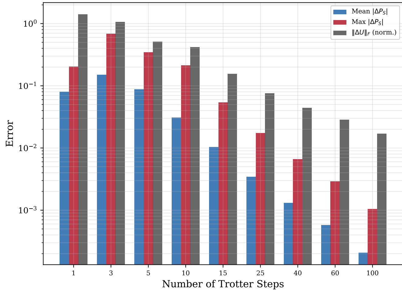
(b) Error Metrics
