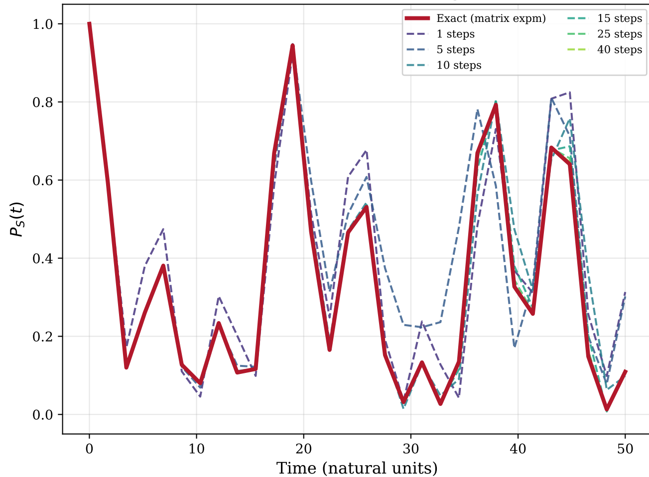
(a) Trotterization Convergence
