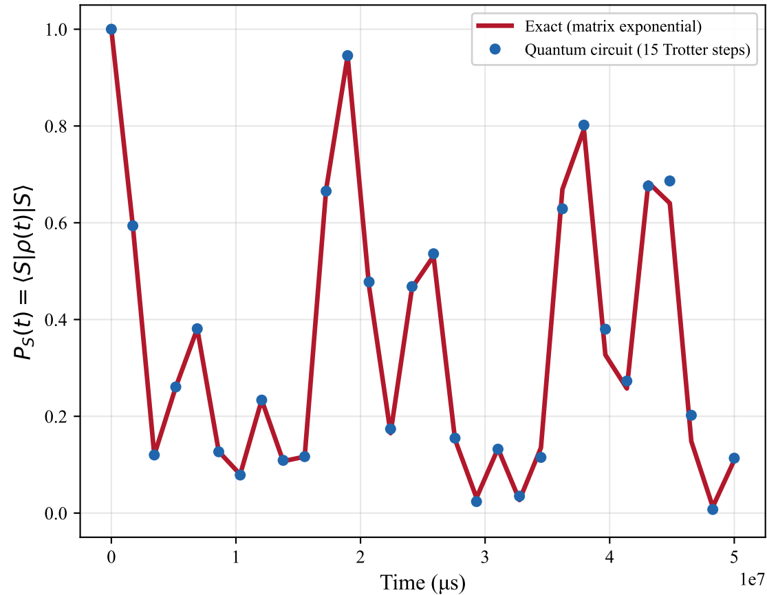
(a) Singlet Probability Evolution [B = 0.1 mT]
