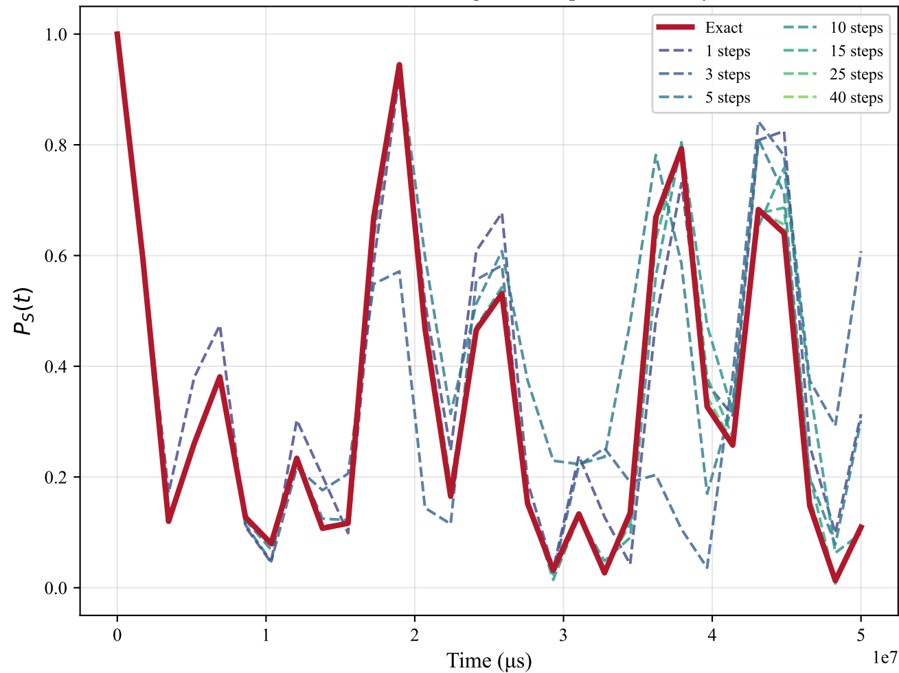
Trotterization Convergence: Steps vs Accuracy
