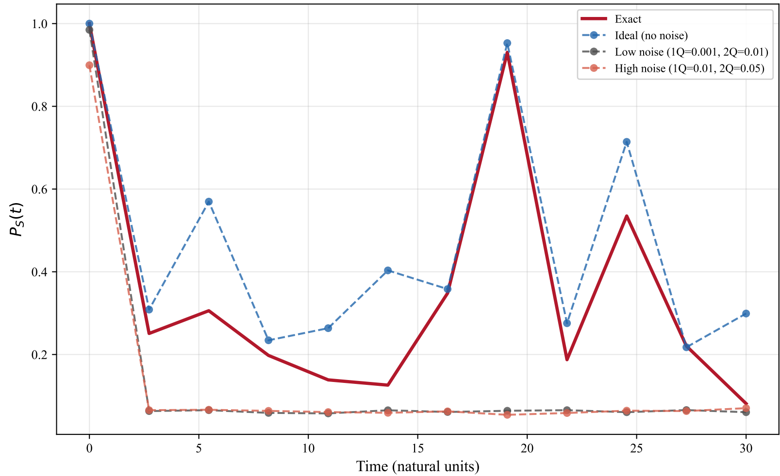
NISQ Noise Effect on RP Quantum Simulation (15 Trotter steps)
