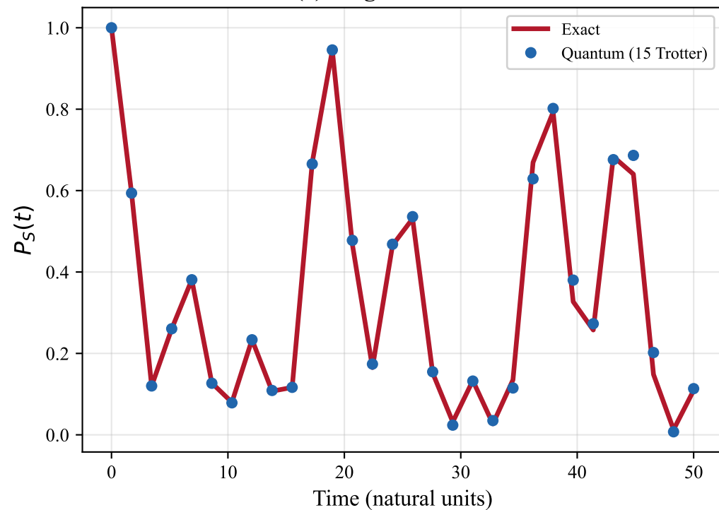
(a) Singlet Evolution
