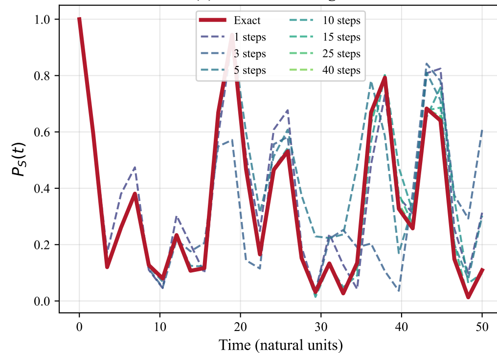
(b) Trotter Convergence
