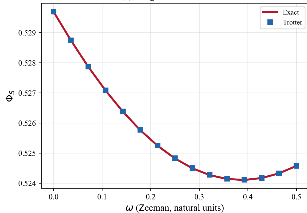
(c) Magnetic Field Effect
