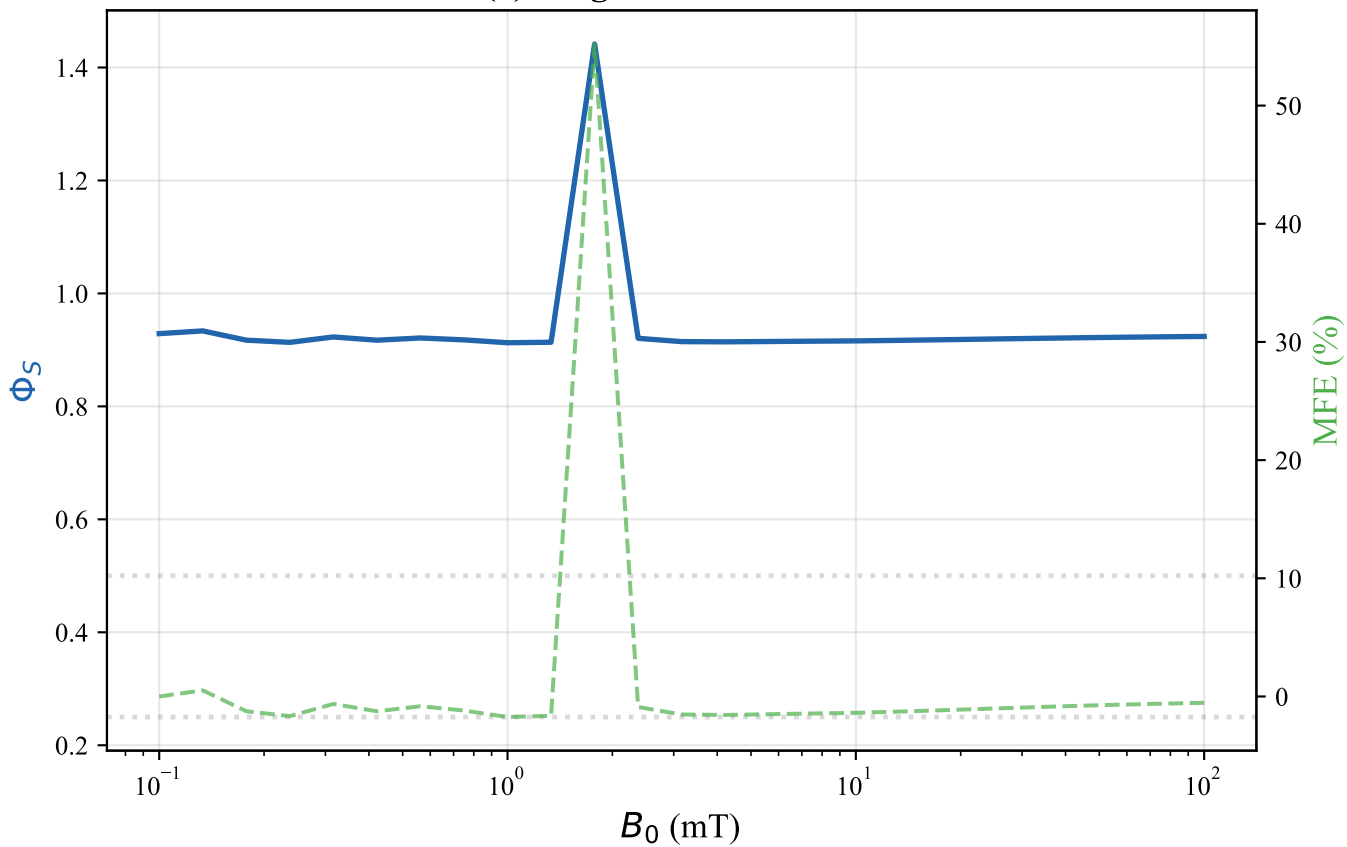
(c) Decoherence Effect
