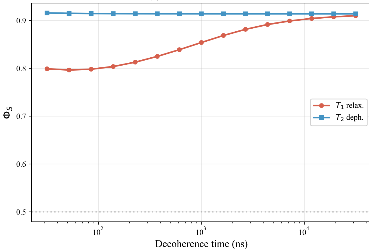
(c) Decoherence Effect
