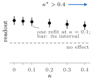
a real at every \kappa
