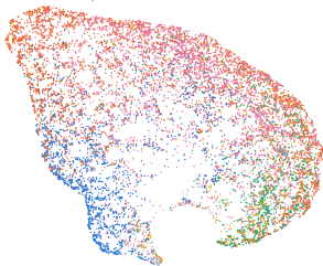
d \mu_w , T/NK cells: neighbours
