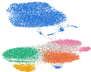
a \mu_z , all cells: own type
