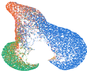
b \mu_w , all cells: neighbours
