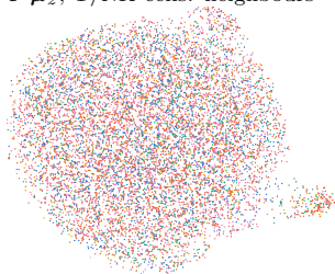
c \mu_z , T/NK cells: neighbours
