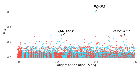
Figure 3. Putative loci under positive selection. AMOVA-corrected F_{ST} -values of SNPs versus alignment position, highlighting the three genes that our SNPs map to, as well as an outlier SNP nearby to PLA2G7 (*), and the outlier SNP which is adjacent to CGMP-PK1 (†). The dashed line marks the significance threshold and alternating colors indicate different genomic scaffolds (1,214 in our dataset).
