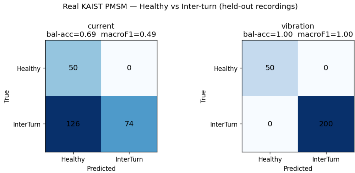
Figure 2: Figure 8.1 — Confusion matrices for the current and vibration channels.
