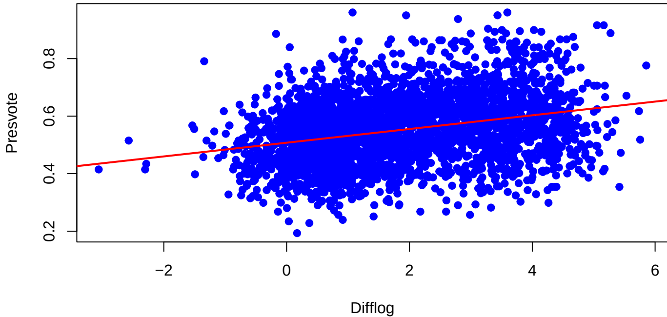
Scatterplot of Presvote vs Difflog
