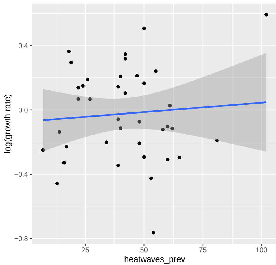
C Effect of heatwaves_prev on growth rate
