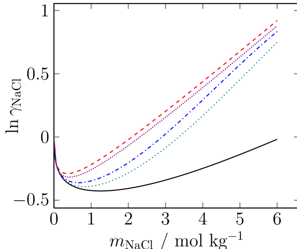
Figure 5: Mean ionic activity coefficient of NaCl over the salt molality for aqueous NaCl solutions at T = 298.15 K using the SPC/E + Joung-Cheatham [33] model combination. The colored lines represent simulation results by different groups for that model combination (from top to bottom): OPAS simulations by Kohns et al. [32] (red dashed line), free energy calculations by Benavides et al. [34] (violet densely-dotted line), gradual insertion of ion pairs by Mester and Panagiotopoulos [30] (blue dashed-dotted line), and osmotic ensemble Monte Carlo simulations by Moučka et al. [31] (green dotted line). The black solid line shows the correlation to experimental data by Hamer and Wu [35].
