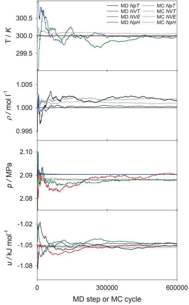
Figure 1: Comparison of the ensembles implemented in ms2 for methyl fluoride (R41)[6] in terms of running averages for temperature T , density \rho , pressure p and potential energy u . Running averages were estimated with the method of Flyvbjerg and Petersen [7].
