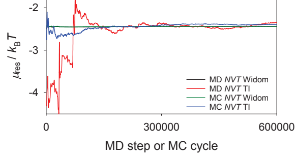
Figure 2: Comparison for the residual chemical potential \mu of methyl fluoride (R41)[6] at T = 300 K and \rho = 20 mol/l calculated by ms2 using either Widom’s particle insertion method (Widom) or the present thermodynamic integration method (TI). Running averages were estimated with the method of Flyvbjerg and Petersen [7].
