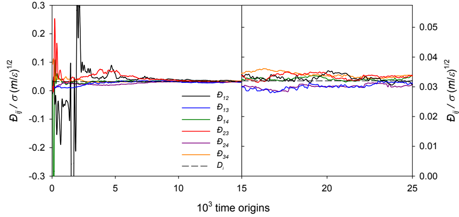
Figure 1: Maxwell-Stefan diffusion coefficients as a function of time origin for the Argon quaternary pseudo mixture at T^* = 0.728 and \rho^* = 0.8442 .
