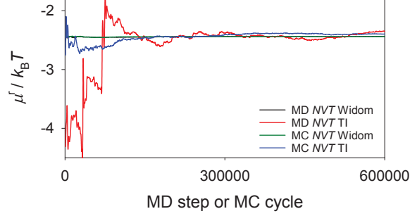
Figure 2: Comparison for the residual chemical potential \mu^r of methyl fluoride (R41)[6] at T = 300 K and \rho = 20 mol/l calculated by ms2 using either Widom’s particle insertion method (Widom) or the present thermodynamic integration method (TI). Running averages were estimated with the method of Flyvbjerg and Petersen [7].
