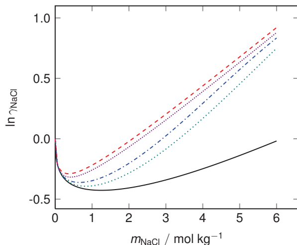
Figure 5: Mean ionic activity coefficient of NaCl over salt molality for aqueous NaCl solutions at T = 298.15 K and p = 1 bar using the SPC/E + Joung-Cheatham [33] model combination. The colored lines represent simulation results by different groups for that model combination (from top to bottom): OPAS simulations by Kohns et al. [32] (red dashed line), free energy calculations by Benavides et al. [34] (violet densely-dotted line), gradual insertion of ion pairs by Mester and Panagiotopoulos [30] (blue dashed-dotted line), and osmotic ensemble Monte Carlo simulations by Moučka et al. [31] (green dotted line). The black solid line shows the correlation to experimental data by Hamer and Wu [35].
