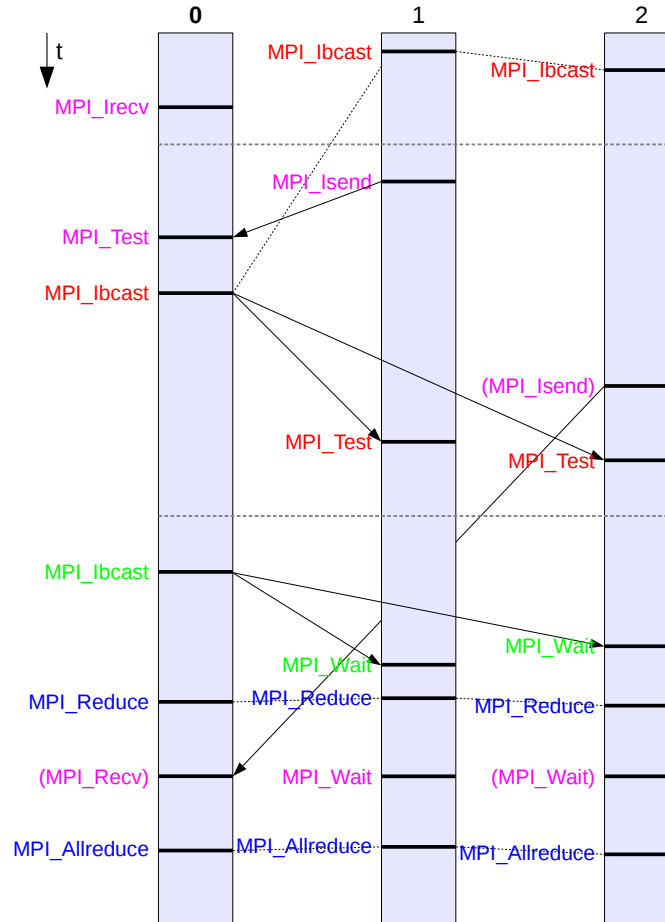
Figure 7: ms2 communication to pass termination status to all PEs
