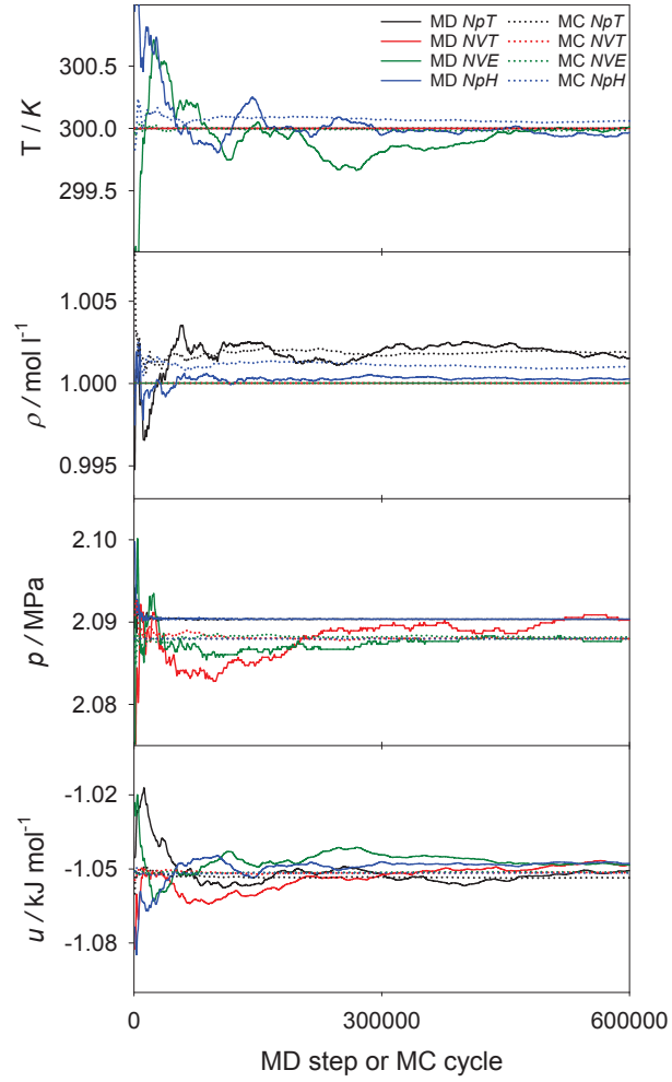
Figure 1: Comparison of the ensembles implemented in ms2 for methyl fluoride (R41) [6] in terms of running averages for temperature T , density \rho , pressure p and potential energy u .
