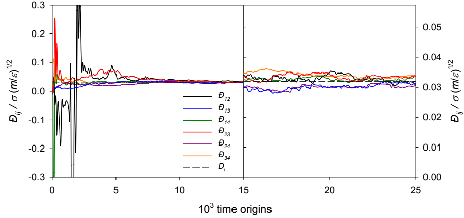
Figure 3: Maxwell-Stefan diffusion coefficients \mathcal{D}_{ij} as a function of time origins for a quaternary pseudo mixture ( \epsilon = \epsilon_1 = \epsilon_2 = \epsilon_3 = \epsilon_4 and \sigma = \sigma_1 = \sigma_2 = \sigma_3 = \sigma_4 ) at k_B T / \epsilon = 0.728 and \rho \sigma^3 = 0.8442 .
