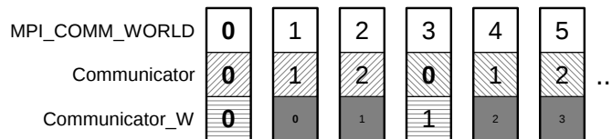
Figure 5: ms2 MPI ranks
