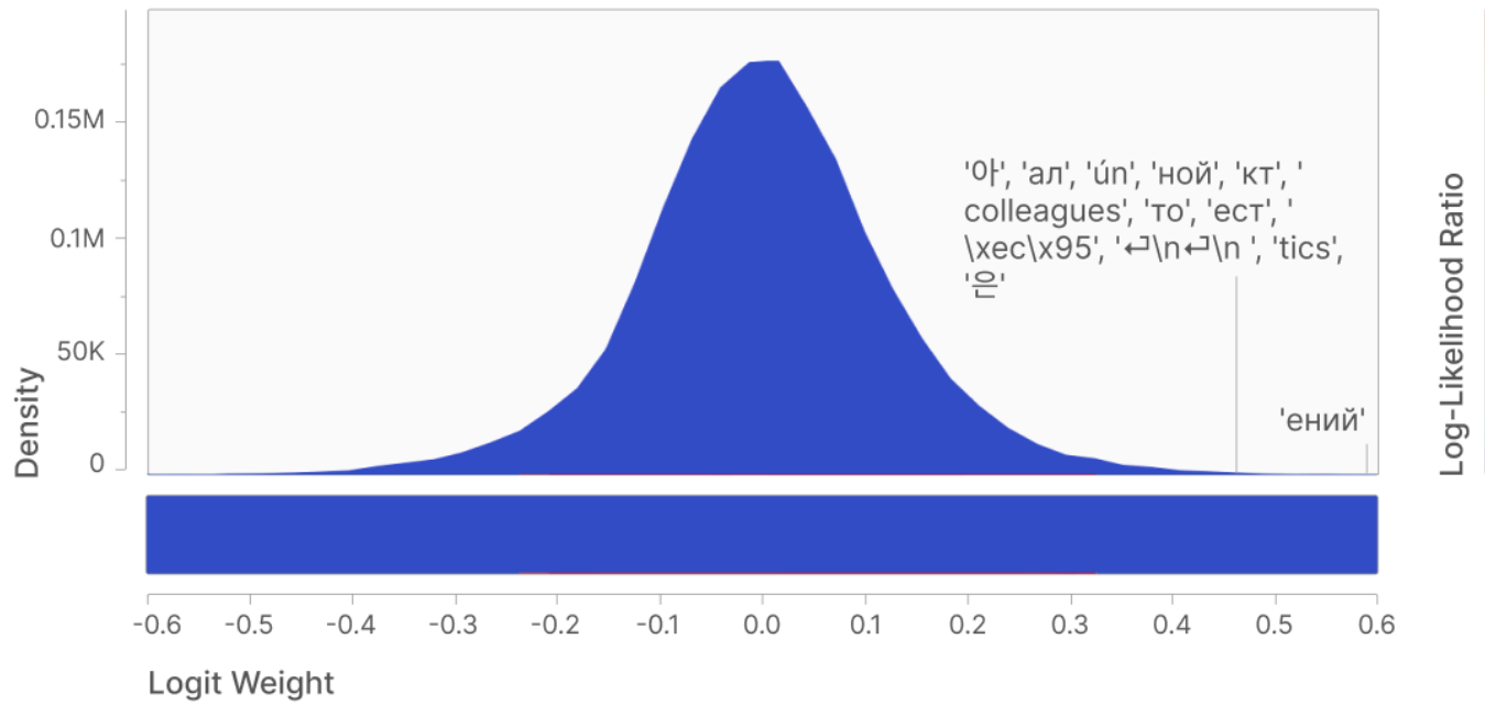
Distribution of Logit Weights (A/neuron/489)
