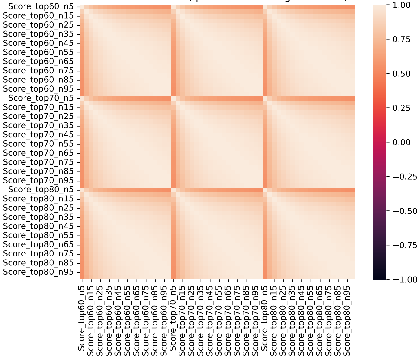
Feature correlations (quantile-based neighbourhood)
