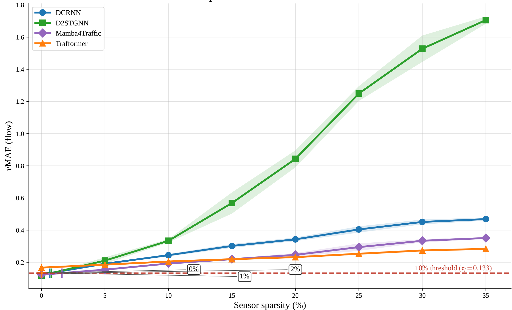
PEMS04: operational breakdown — flow channel
