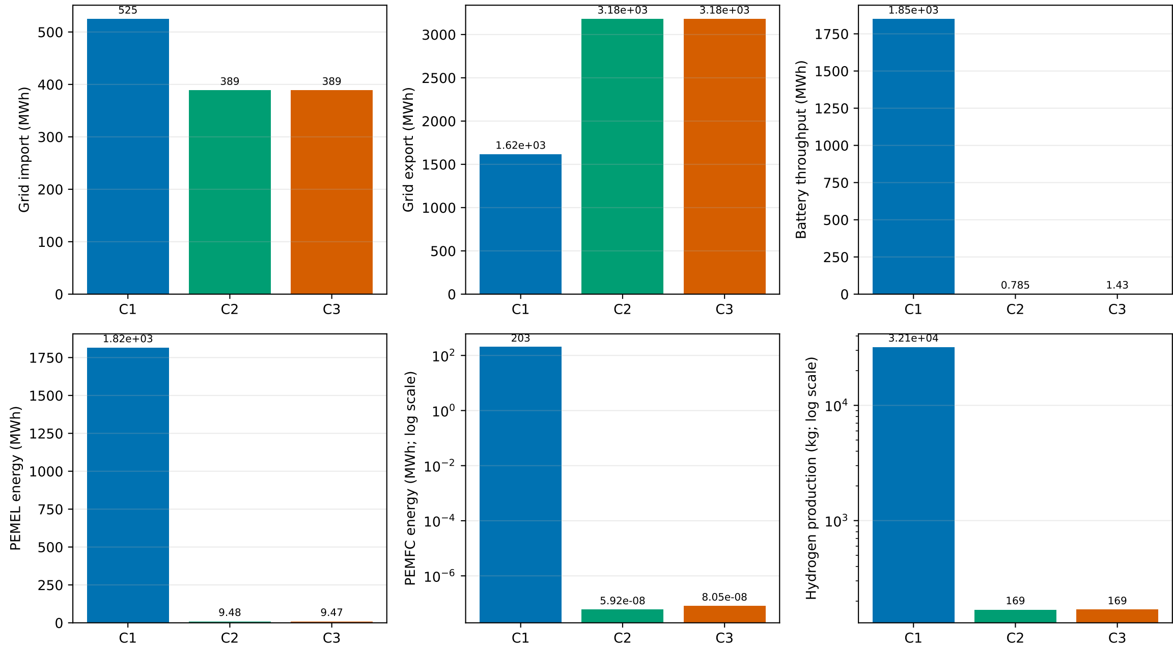
Annual operating regimes under the fixed PV-rich case
