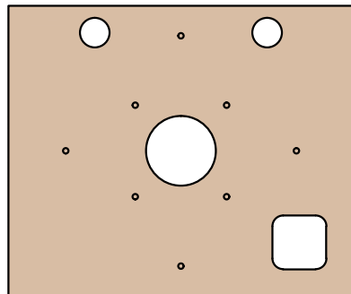
FIREWALL & CONTROL HORN 1/16" (1.5mm) THICK HOBBY GRADE PLYWOOD
