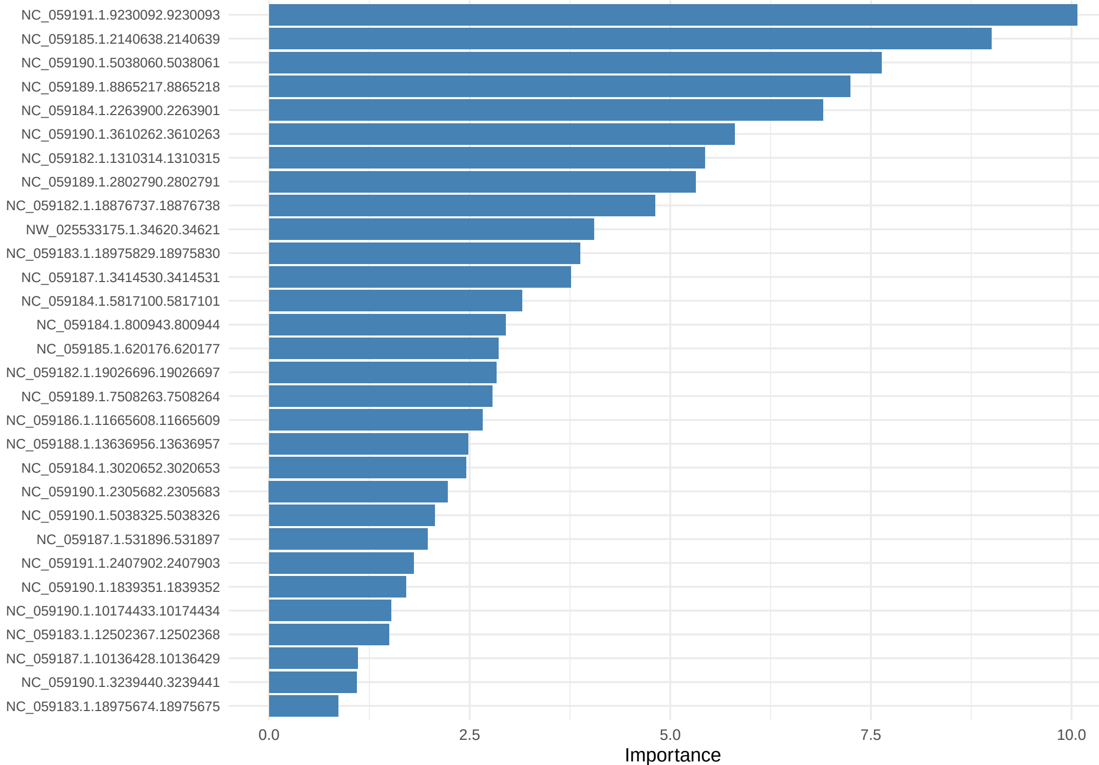
Pesticide Lvl Feature Importance (Top 30)
