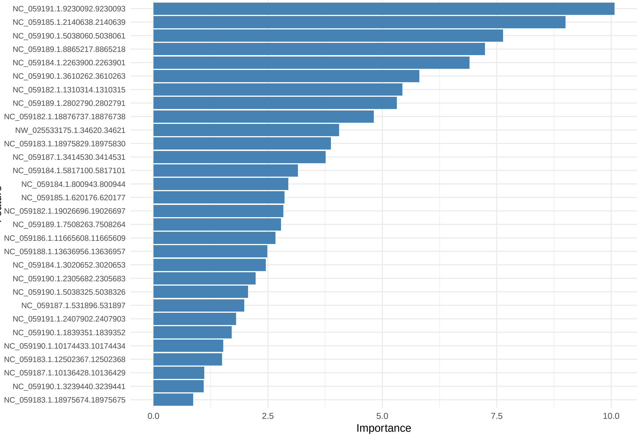
Pesticide Lvl Feature Importance (Top 30)
