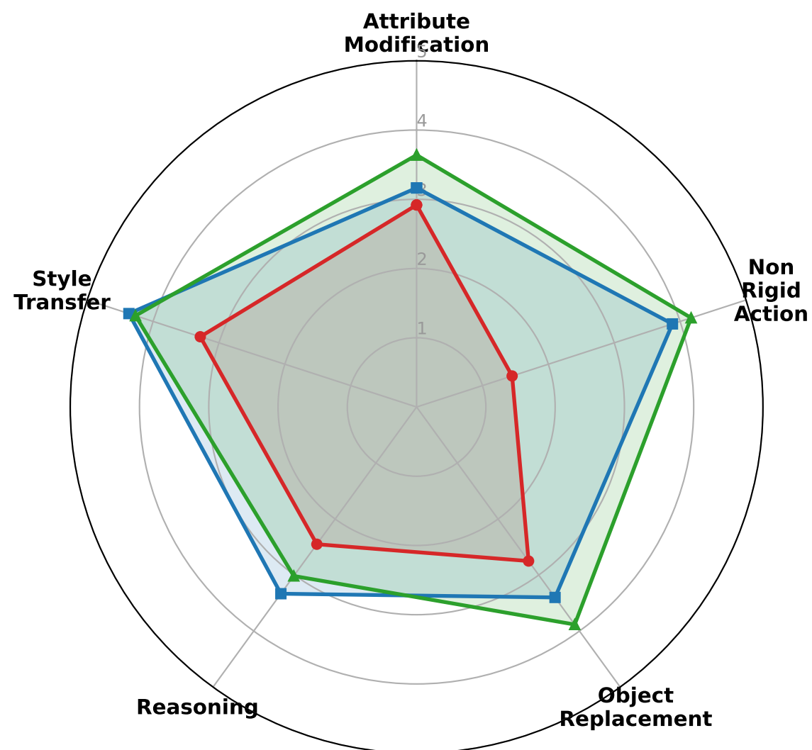
Pix2Pix-Zero
