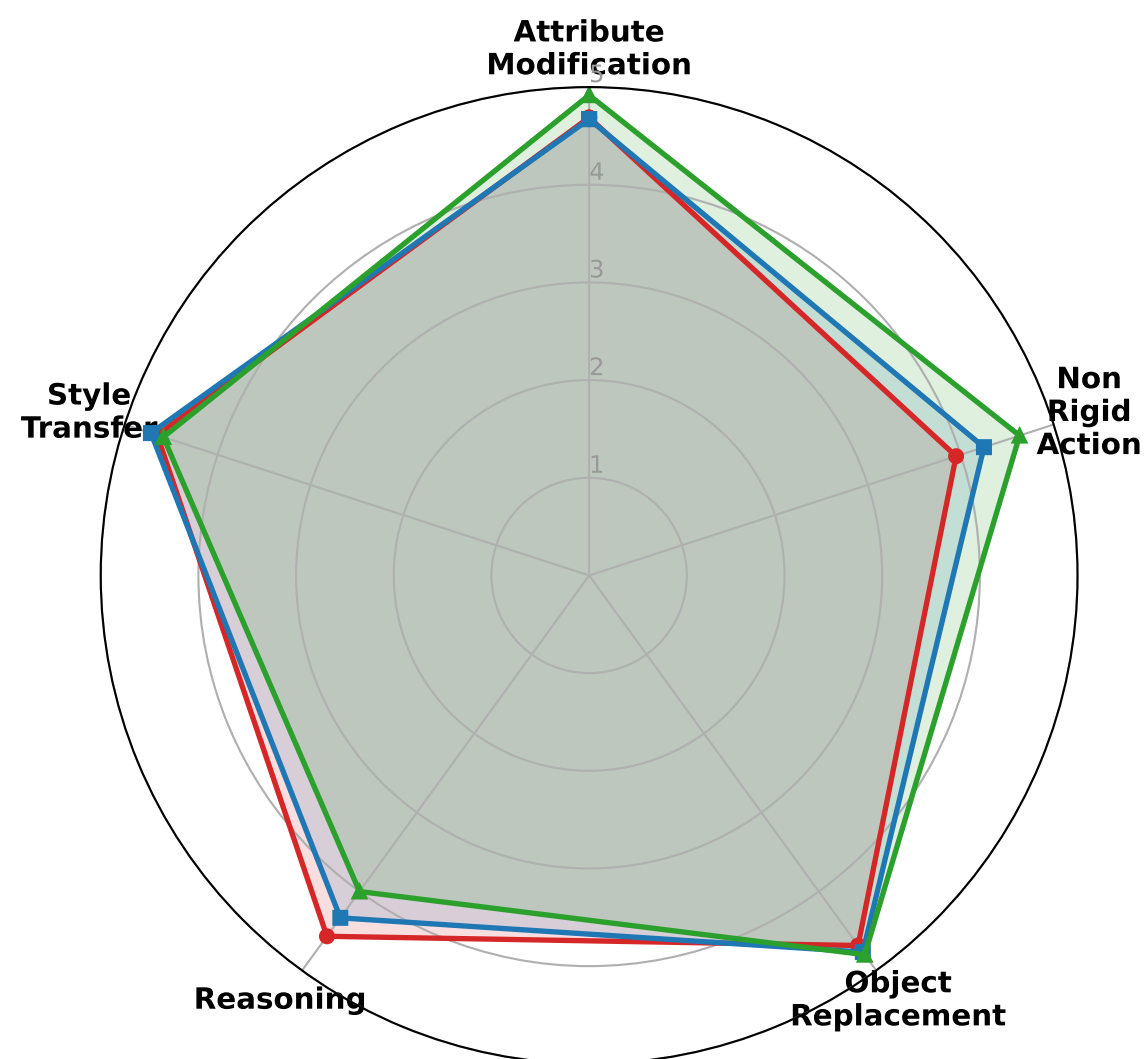
Qwen-Edit
