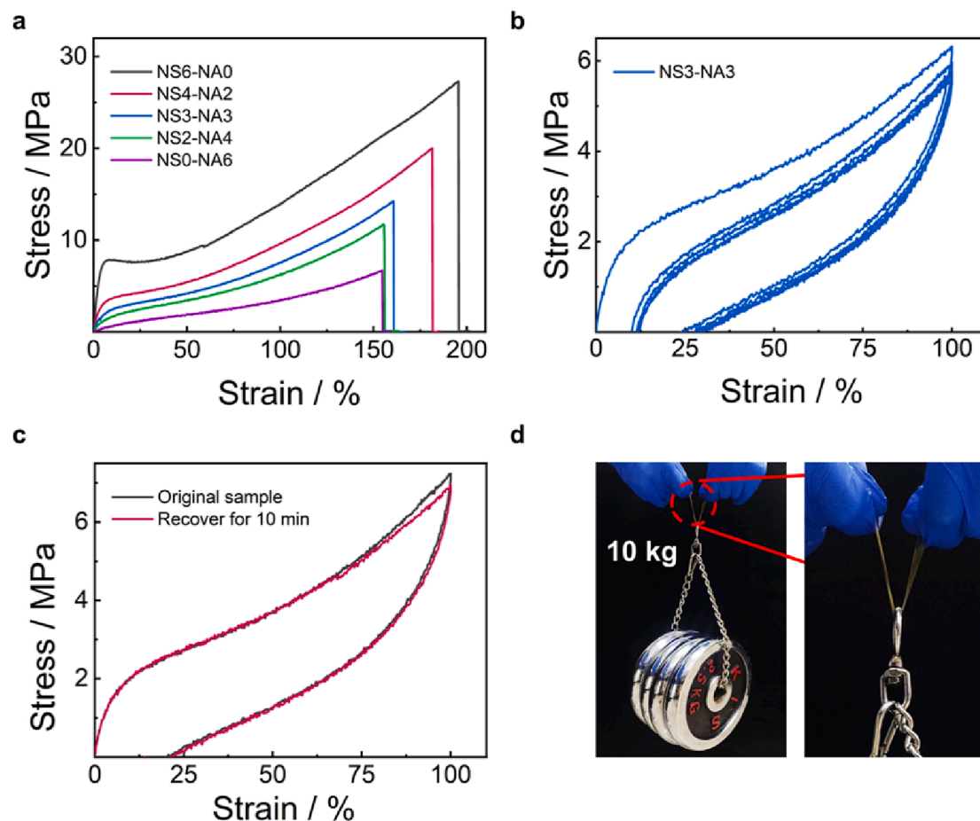
Fig. 1. (a) Stress–strain curves of NSx–NAy. (b) Cyclic stretch curve of NS3–NA3. (c) Cyclic stretch curves of NS3–NA3 at the initial state and after a ten-minute recovery. (d) Demonstration of the load bearing of NS3–NA3.
