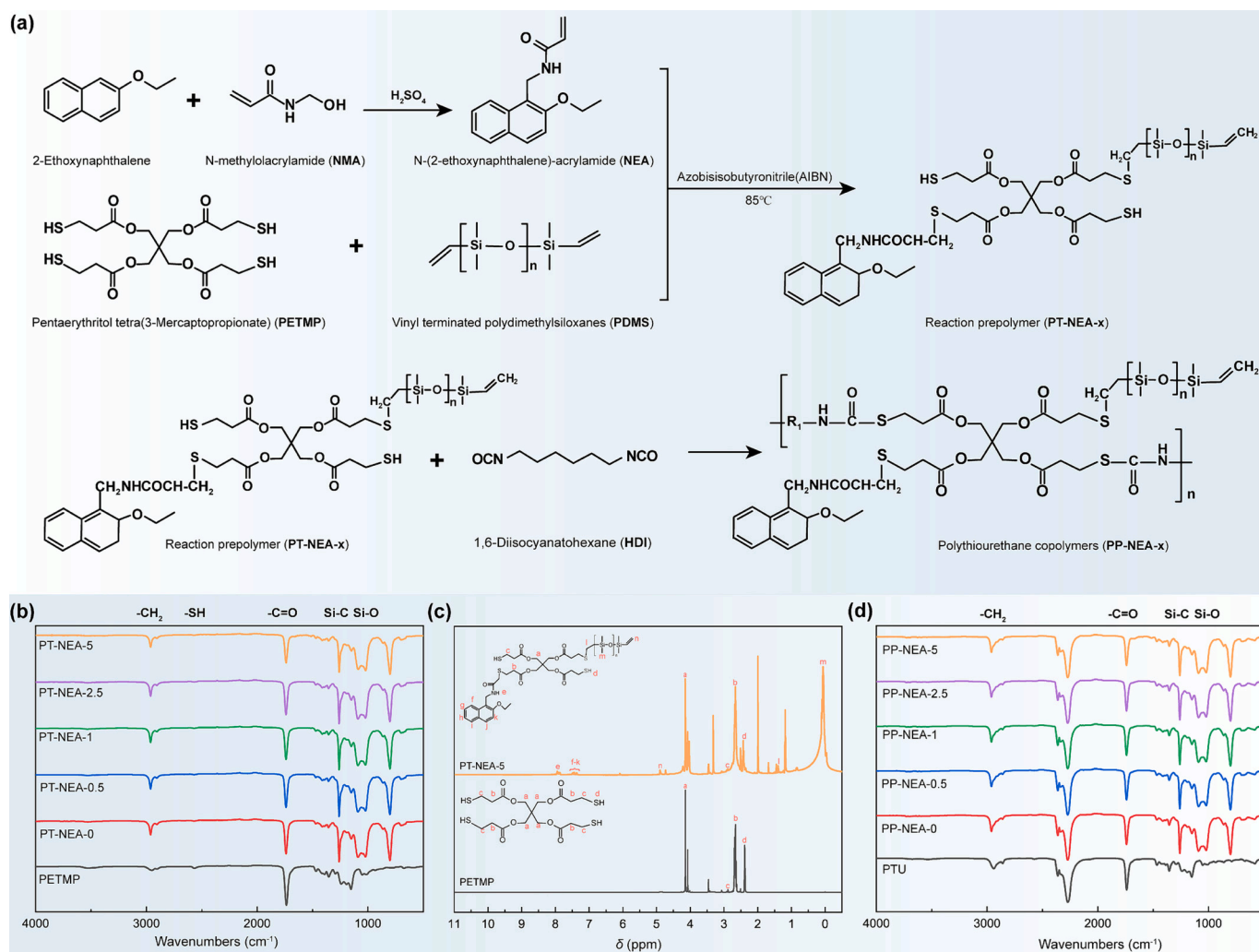
Fig. 1. (a) Synthesis process of nature-inspired silicone-polythiourethane coatings based on capsaicin analogue; (b) FT-IR spectra of PETMP and PT-NEA-x; (c) ^1\text{H} NMR spectra of PETMP and PT-NEA-5; (d) FT-IR spectra of PTU and PP-NEA-x.
