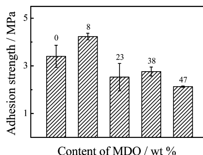
Figure 1. Adhesion strength of PMSMx with different MDO content.
