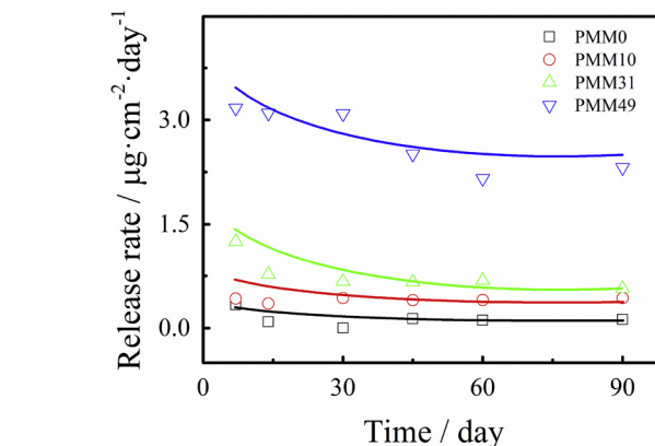
Fig. 5. Time dependence of the release rate of DCOIT from PMMx in ASW at 25 °C.
