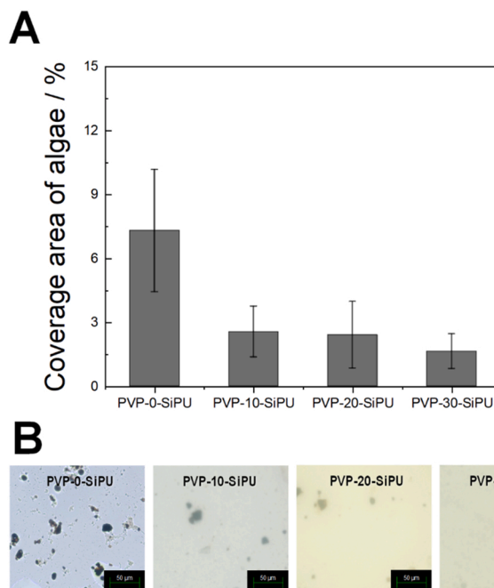
Fig. 6. Algae inoculation test after 7 days of culture (A) Percentage of algae coverage on different coatings and (B) Representative microscopic images of different coatings.
