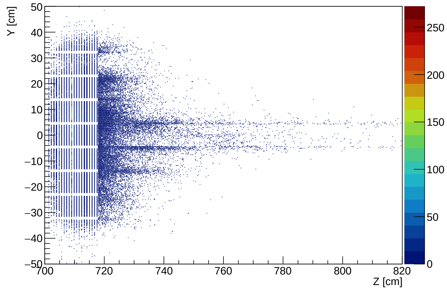
Hit map in YZ plane
