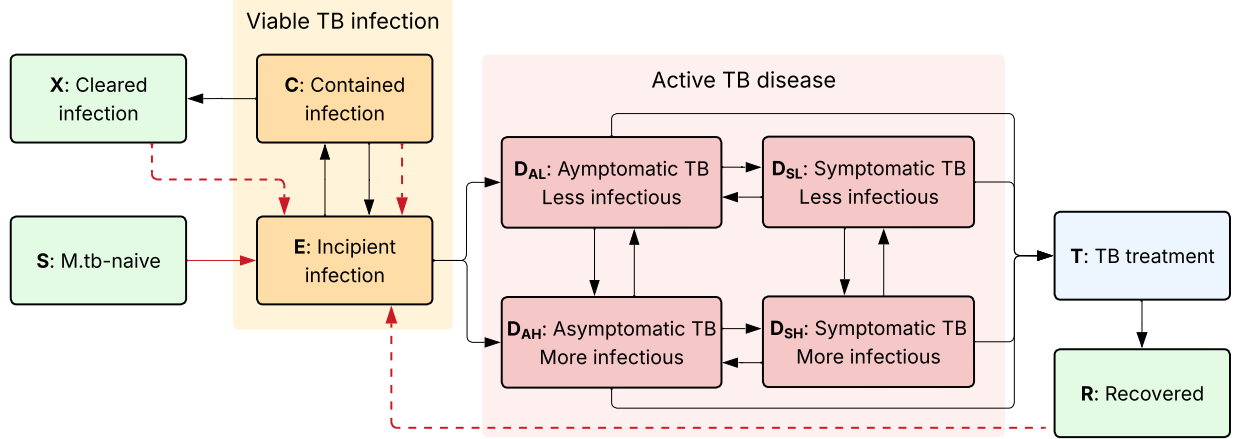
Figure 1: Schematic of model compartments and transitions. Transmission pathways are shown in red, with dashed red arrows indicating reinfection. For clarity, age and screening-reachability stratification, births, natural mortality, spontaneous recovery from asymptomatic TB, and TB-related mortality from symptomatic TB are not shown.
