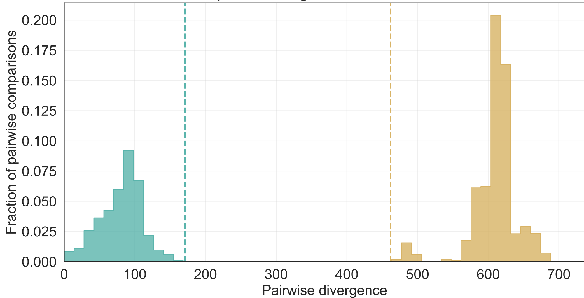
Distribution of NA pairwise divergences for North American avian viruses
