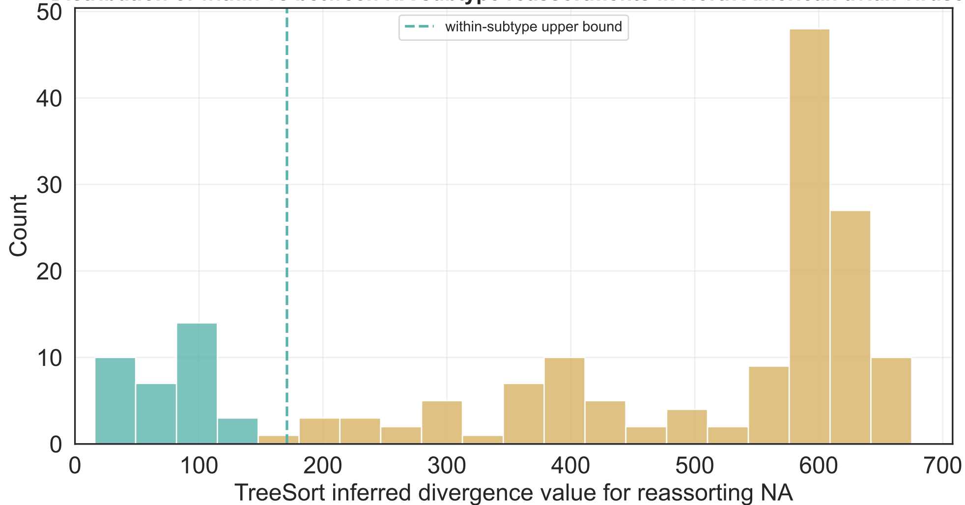
Distribution of within vs between NA subtype reassortments in North American avian viruses
