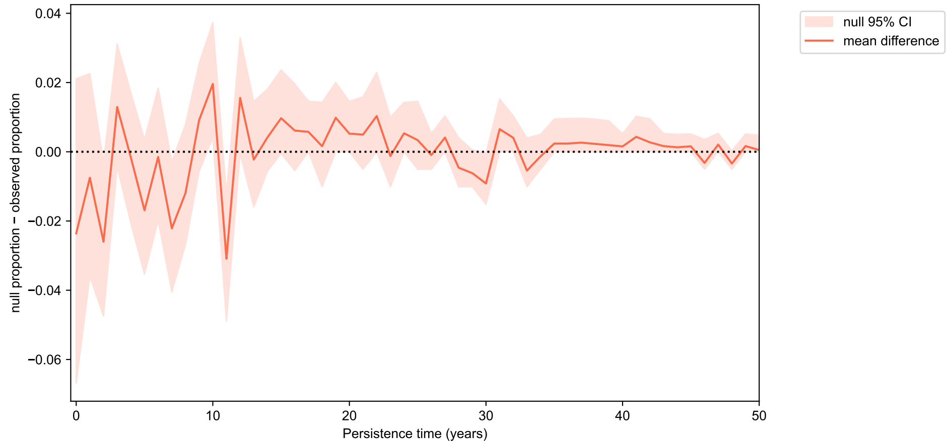
eurasian_avian persistences
