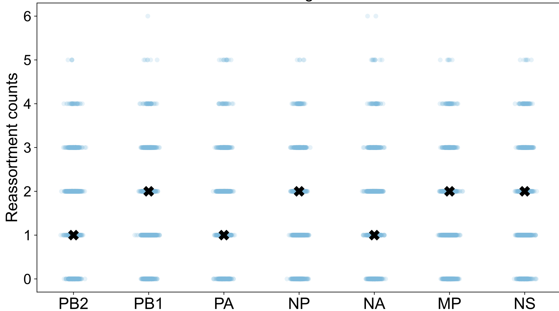
Simulated vs observed segment counts for canine
