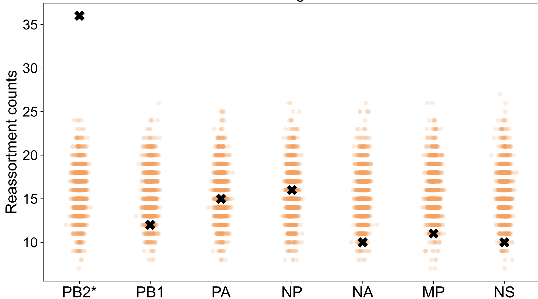
Simulated vs observed segment counts for human
