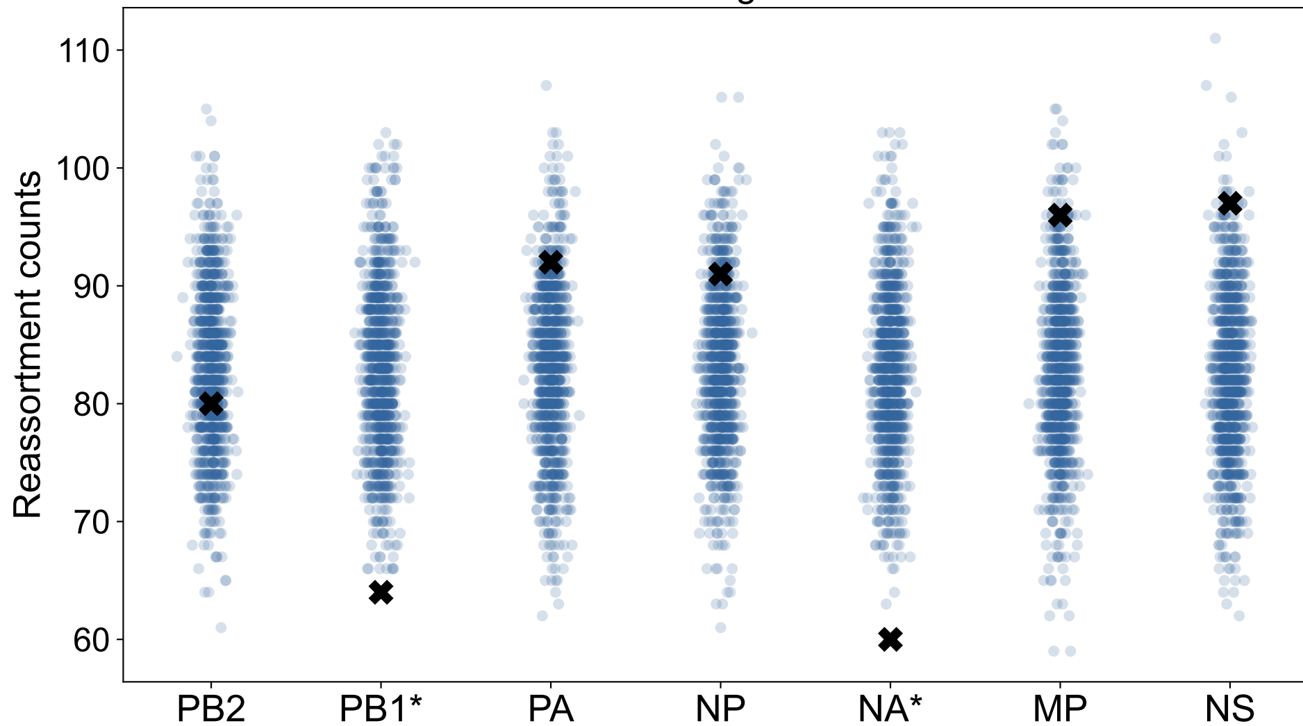
Simulated vs observed segment counts for swine
