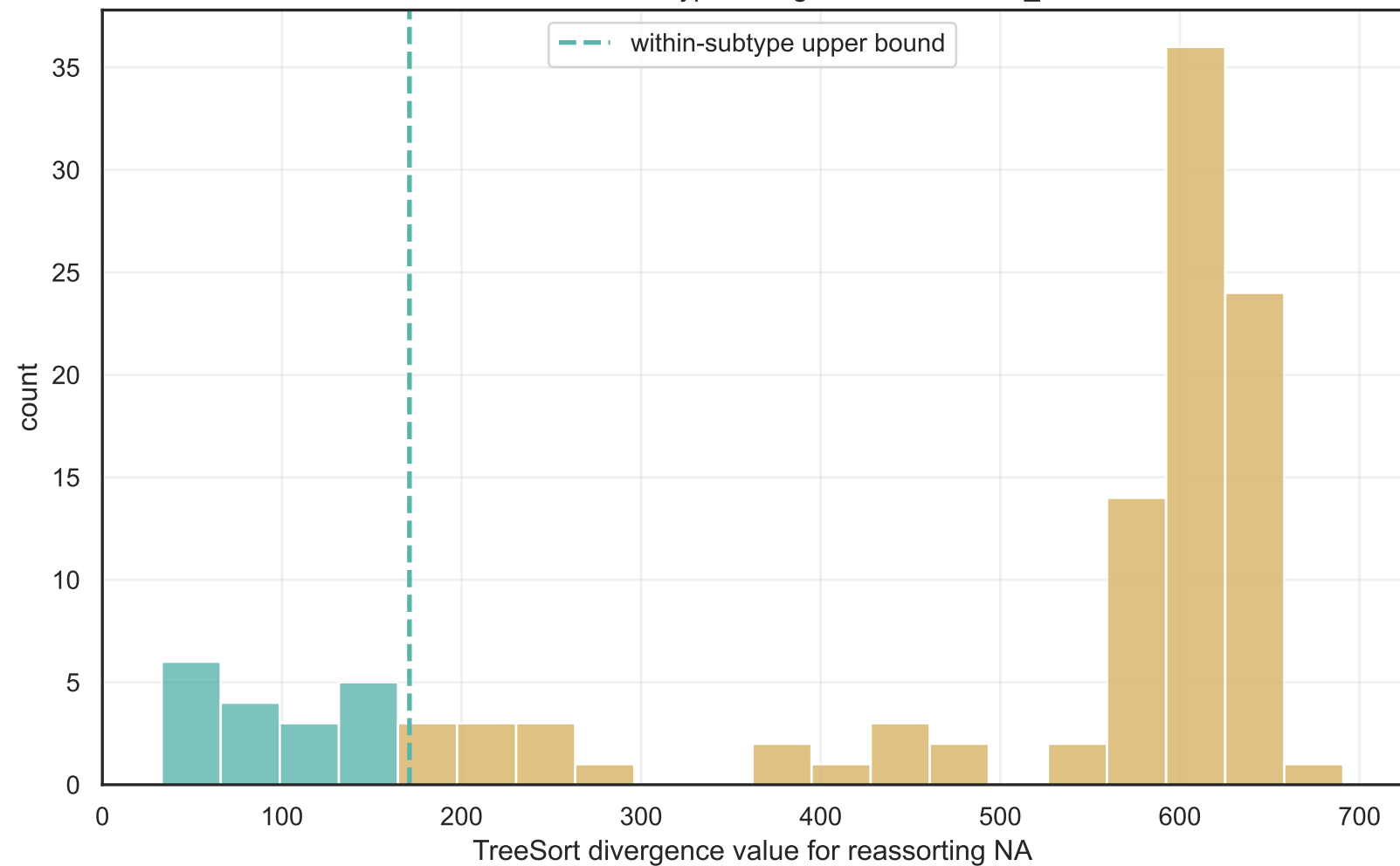
within vs between subtype divergence for eurasian_avian
