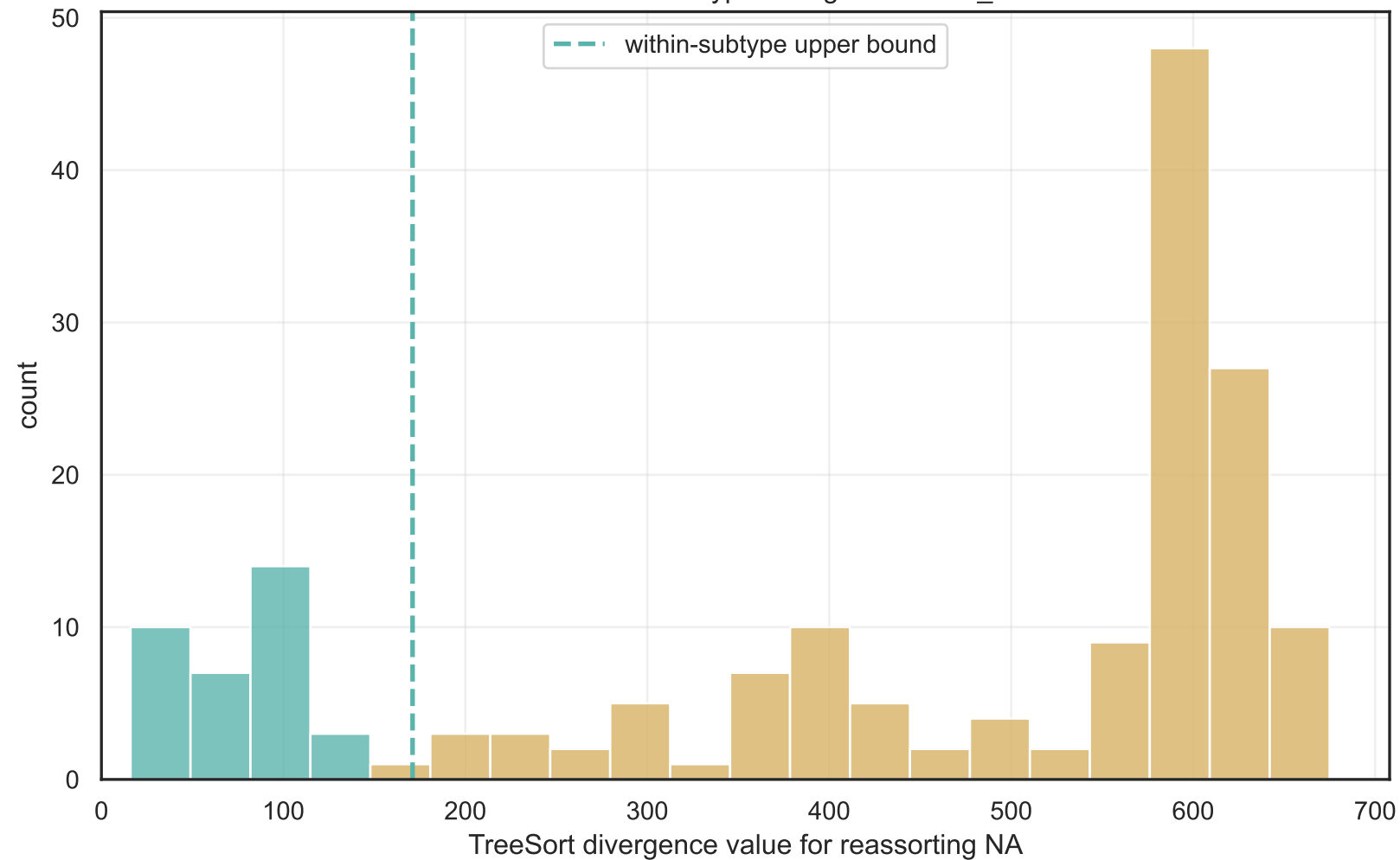
within vs between subtype divergence for na_avian
