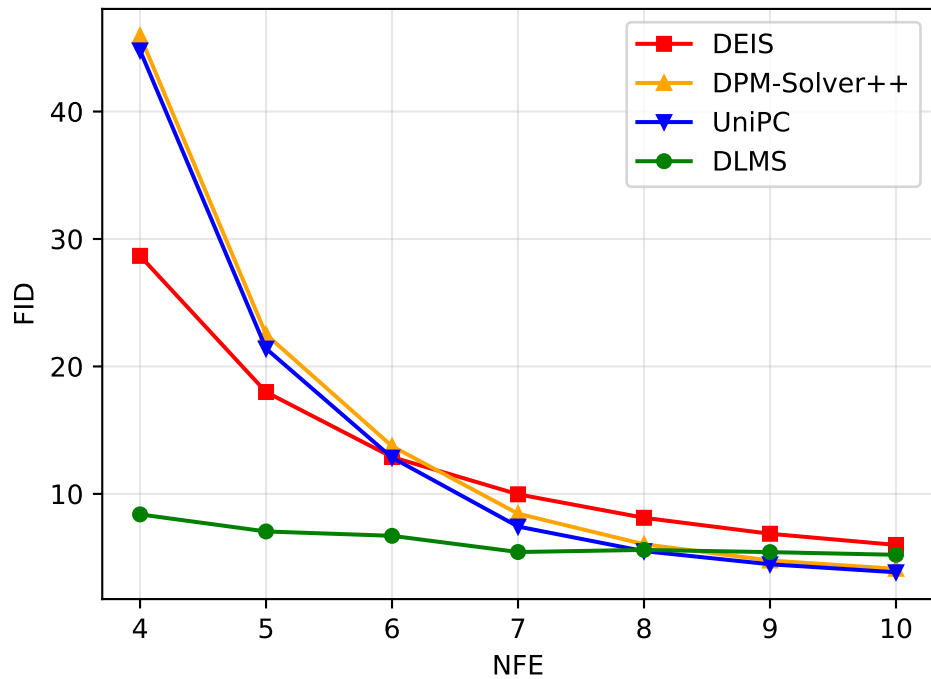
FFHQ 64×64 (pixel space, unconditional)
