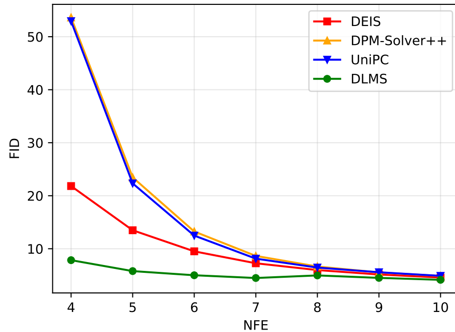
ImageNet-64 64×64 (pixel space, conditional)
